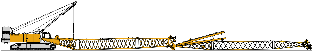
Assembly of boom
